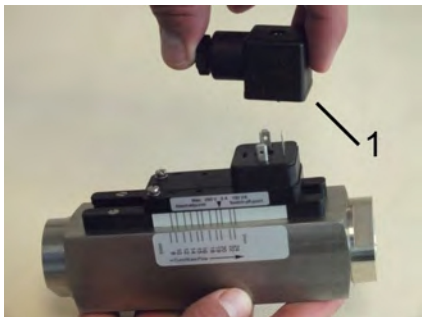
Fig. 52: Remove female socket
