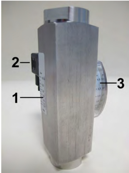
Fig. 1: SW-06 flow monitor
