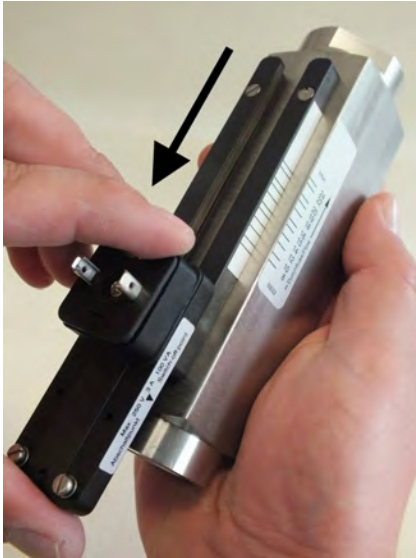
Fig. 54: Remove the switch contact from guide rails
