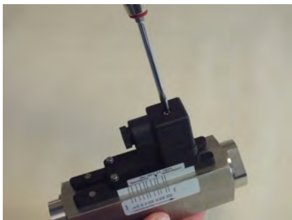
Fig. 51: Loosen female socket
