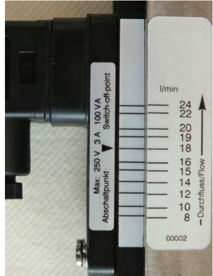
Fig. 4: Scale on the device body SW-06
