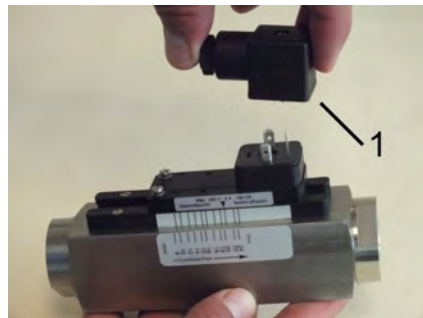
Fig. 22: Remove socket
