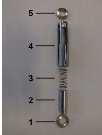
Fig. 38: Inner parts SW-06
