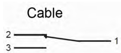
Fig. 18: Pin-assignment, socket M12x1 Form 30x70)
