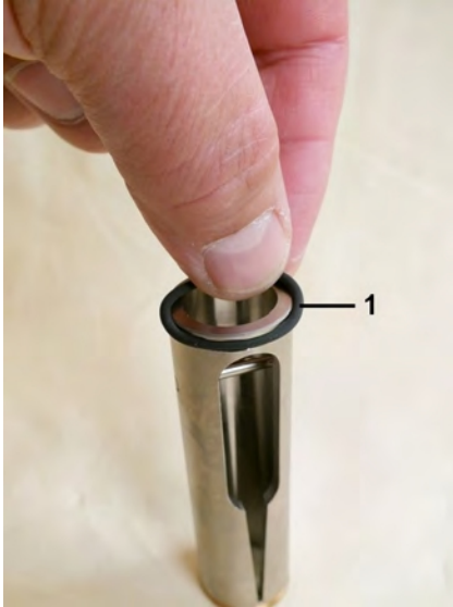
Fig. 43: O-ring (centering the slot nozzle)
