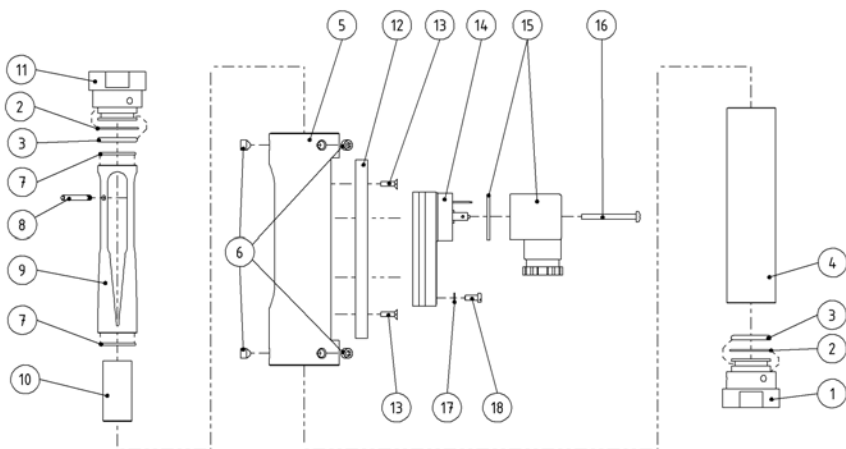
Fig. 65: Spare parts drawing
