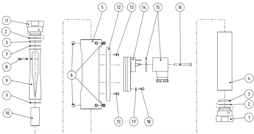
Fig. 64: Replacement parts drawing
