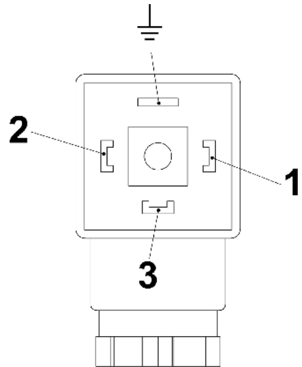
Fig. 24: Pin assignment, plug socket, change-over contact (Form 30x70)
