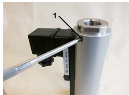
Fig. 33: Loosen screws
