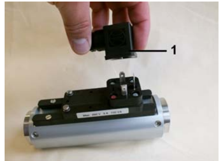
Fig. 56: Remove the female socket
