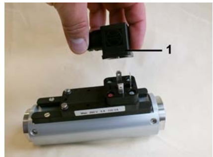
Fig. 20: Remove socket
