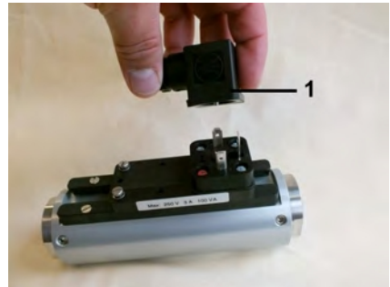
Fig. 57: Remove the female socket
